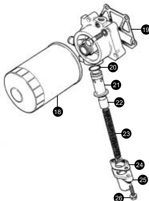
Late S2 & S3 Spin-Off Oil Filter
