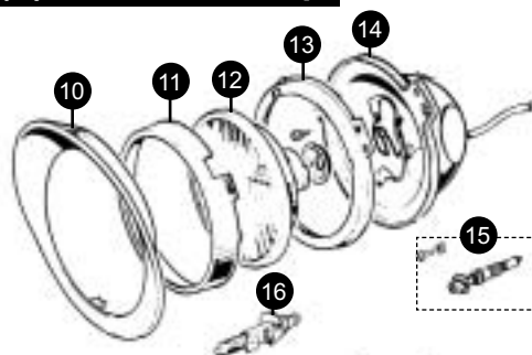
(B) 5.75" Headlamp
