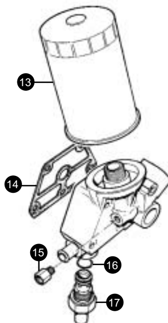
Early S2 Spin-Off Oil Filter
